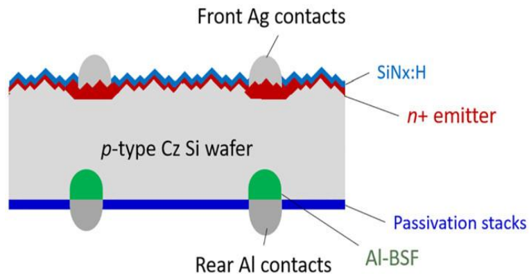
PERC solar cell
