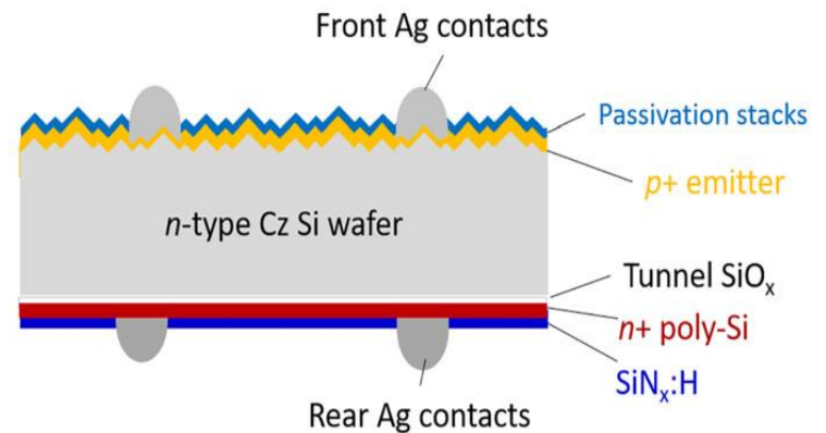
TOPCON solar cell
